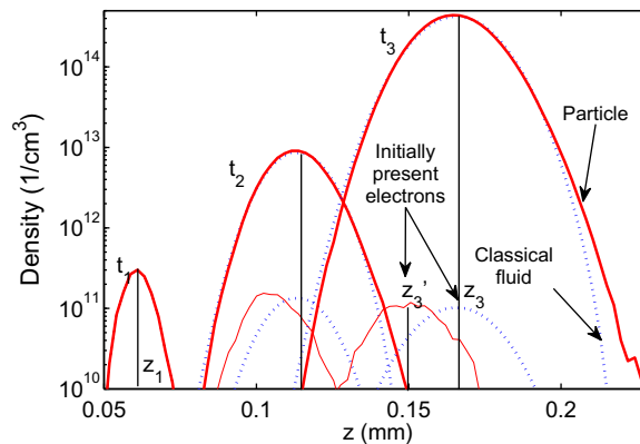
Fig. 3. Evolution of electron swarms at three consecutive time steps t_1, t_2, t_3 in a field of -100 kV/cm, where t_1, t_2, t_3 are 20, 130, 240 ps when the simulation starts from 100 pairs of electrons and ions. Shown are the spatial profiles of the total swarm in the 1D particle model (solid line) and in the 1D classical fluid model (dotted line). Also shown are the spatial profiles of those electrons that were already present at time t_1 (at the same three time steps).
